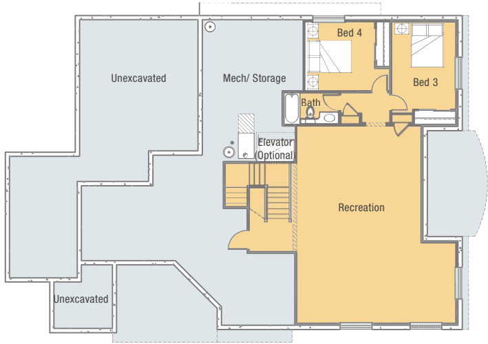
Lower Level Floor Plan – Optional Finish
