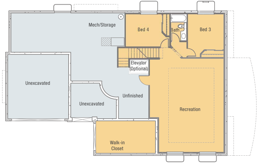
Lower Level Floor Plan – Optional Finish
