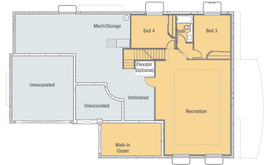
Lower Level Floor Plan – Optional Finish
